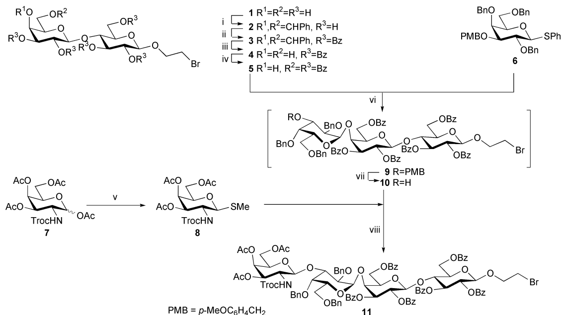
Scheme 1 Reagents and conditions: i, PhCH(OMe) 2 , PTSA, MeCN (89%); ii, BzBr, pyridine, CH 2 Cl 2 (71%); iii, AcOH, water, 80 °C (70%); iv, BzCl, pyridine, CH 2 Cl 2 , -78 °C (82%); v, Me 3 SiMe 2 , Me 3 SiOTf, MS AW-300, (CH 2 Cl) 2 (96%); vi, NIS, TfOH, CH 2 Cl 2 , Et 2 O, MS AW-300, -45 °C; vii, TfOH, 0 °C, 40 min; viii, NIS, 8 , -45 °C (76% for vi–viii one pot).
