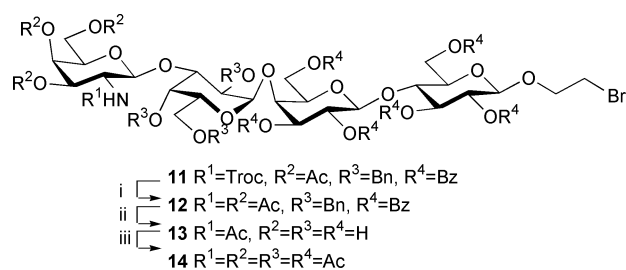
Scheme 2 Reagents: i, ^{\text{a}}\text{Zn} , AcOH; ^{\text{b}}\text{Ac}_2\text{O} , MeOH (86%); ii, ^{\text{a}}\text{H}_2 , Pd/C, AcOH; ^{\text{b}}\text{NaOMe} , MeOH (79%); iii, \text{Ac}_2\text{O} , pyridine, DMAP (88%).
